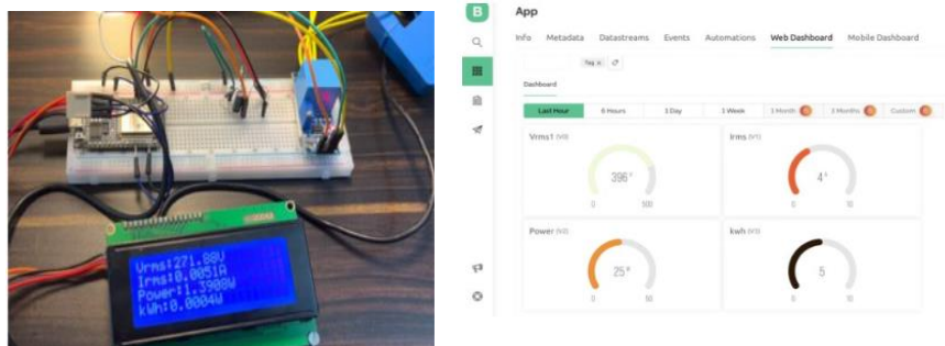
Fig.5 Smart Energy Meter Compact Size Model
