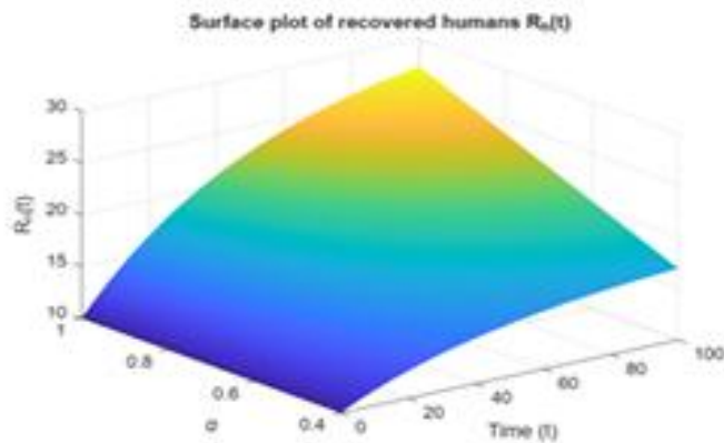
FIGURE 9. Three-dimensional surface of the recovered human population R_h(t) versus the fractional order \alpha and time t .
