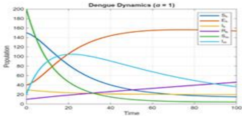
FIGURE 5. Behaviour of the model variables at time t using Fibonacci wavelet with \alpha = 1 .
