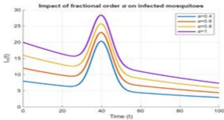
FIGURE 13. Impact of the fractional-order parameter \alpha on the infected mosquito population I_m(t) .
