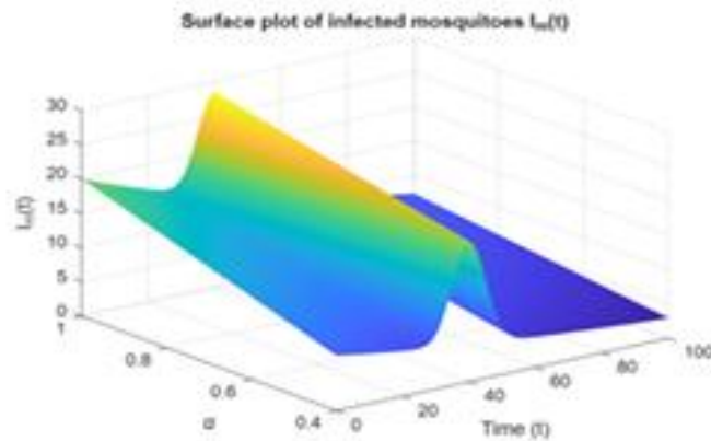
FIGURE 11. Three-dimensional surface of the infected mosquito population I_m(t) versus the fractional order \alpha and time t .
