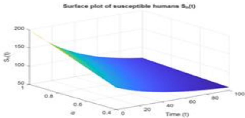
FIGURE 6. Three-dimensional surface of the susceptible human population S_A(t) versus the fractional order \alpha and time t .
