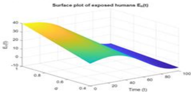
FIGURE 7. Three-dimensional surface of the exposed human population E_A(t) versus the fractional order \alpha and time t .
