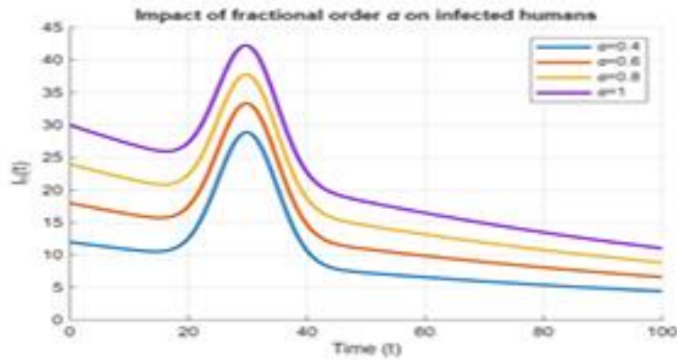
FIGURE 12. Impact of the fractional-order parameter \alpha on the infected human population I_h(t) .
