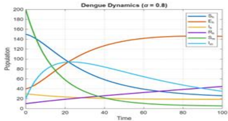
FIGURE 4. Behaviour of the model variables at time t using Fibonacci wavelet with \alpha = 0.8 .
