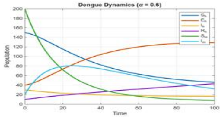
FIGURE 3. Behaviour of the model variables at time t using Fibonacci wavelet with \alpha = 0.6 .
