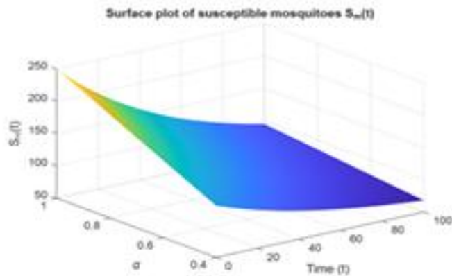
FIGURE 10. Three-dimensional surface of the susceptible mosquito population S_m(t) versus the fractional order \alpha and time t .
