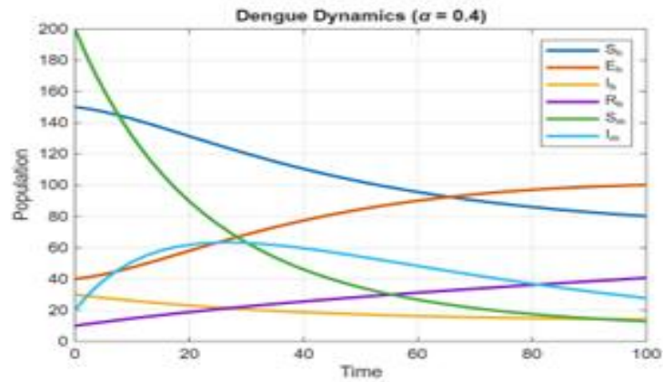
FIGURE 2. Behavior of the model variables at time t using Fibonacci wavelets with \alpha = 0.4 .
