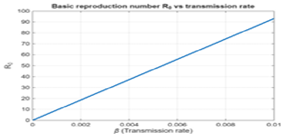
FIGURE 14. Variation of the basic reproduction number R_0 with respect to the transmission rate \beta .
