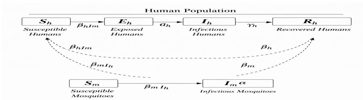
Figure 1. Schematic diagram of the fractional-order dengue transmission model illustrating the interaction between human and mosquito populations.
