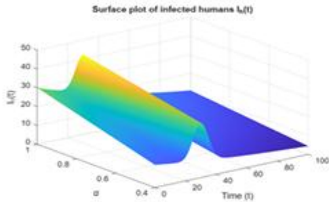
FIGURE 8. Three-dimensional surface of the infected human population I_h(t) versus the fractional order \alpha and time t .
